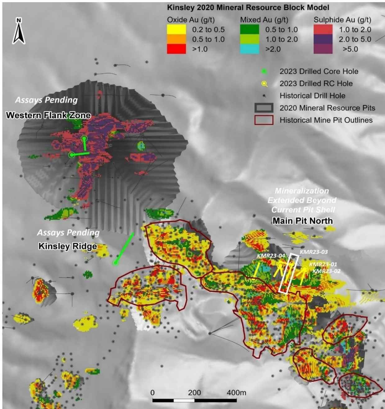
Figure 1. Kinsley Mountain 2023 RC and Diamond Drilling Completed
