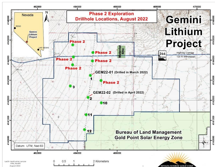
Phase 2 Exploration Program – Drillhole Locations
